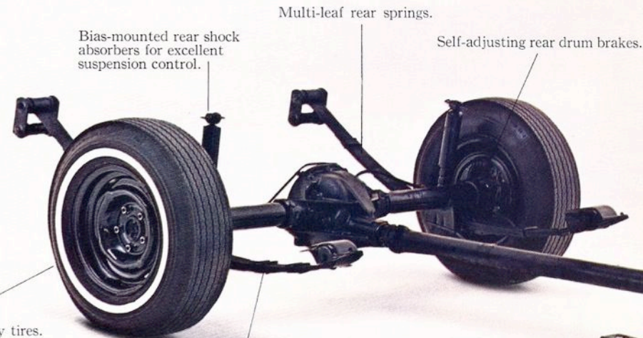
Computer-selected front and rear springs to correspond to equipped weight of car.
