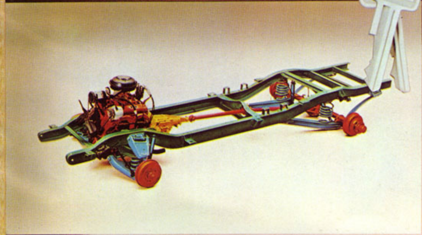
Chassis pg. 14-15
