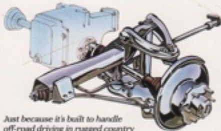
THE DATSUN 4x4 INDEPENDENT FRONT SUSPENSION
