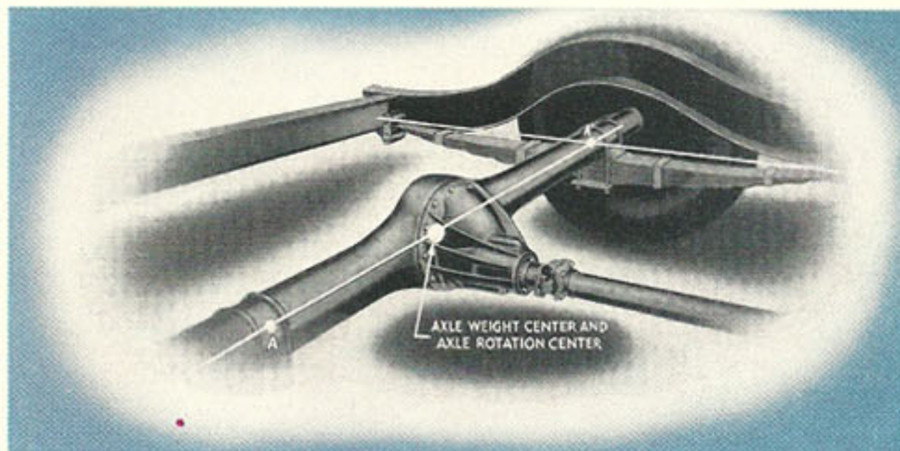
Increased riding comfort has been combined with greater car control by the new Hi-Plane Hotchkiss Drive. Axle vibrations producing body-shake and loss of control are eliminated.
