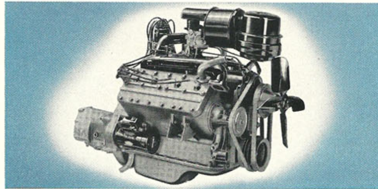
Climaxing a quarter-century of progress in V-type engine design, this 135-horsepower Cadillac engine is unexcelled for its dependability, long life and efficiency of operation.
