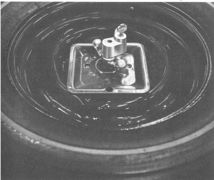
G. Spare Tire Lock ▼
