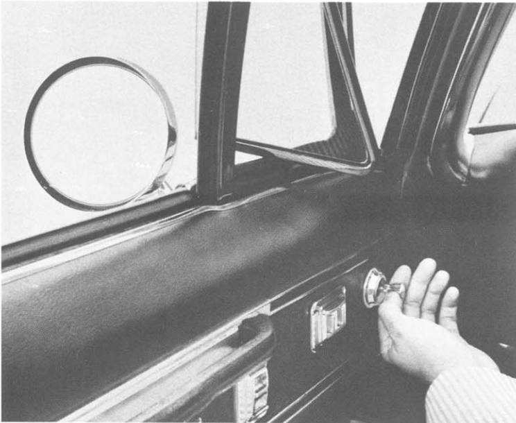
E. Remote Control Outside Mirror ▲
