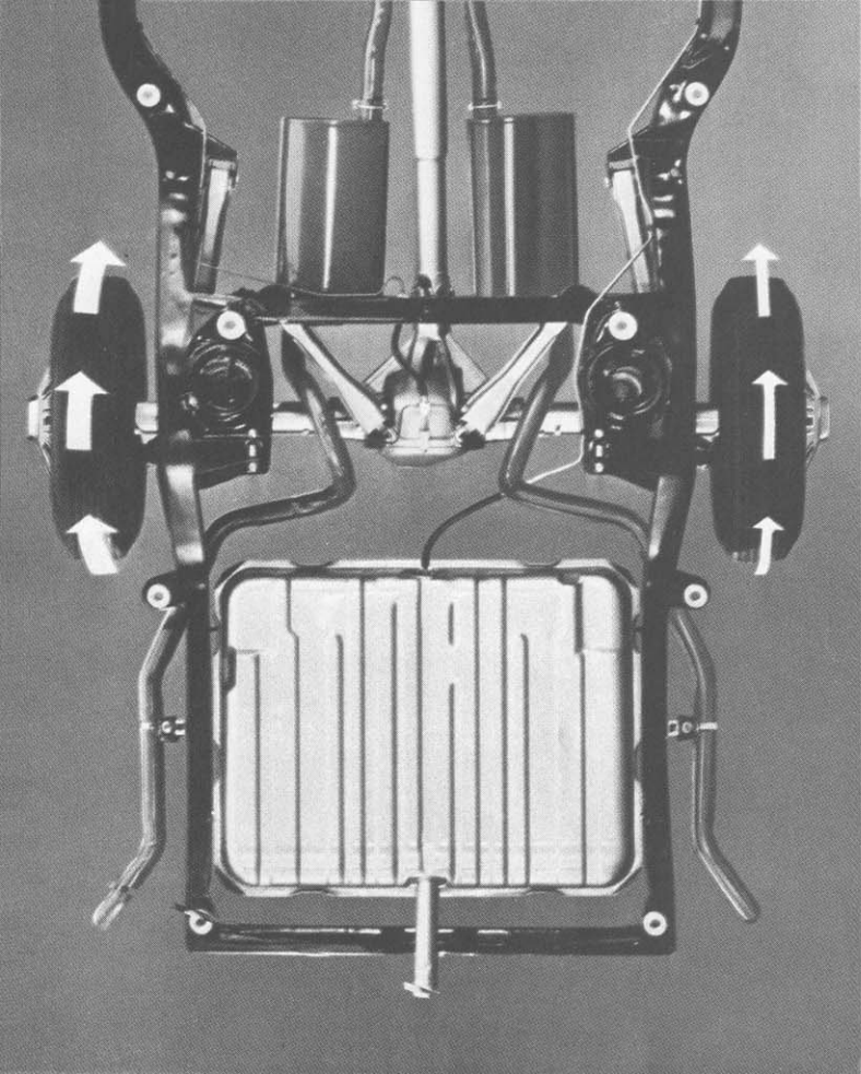
A. Safe-T-Track Differential ▲
