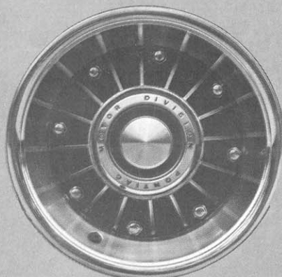
D. Aluminum Wheel Hub and Drums ▲
