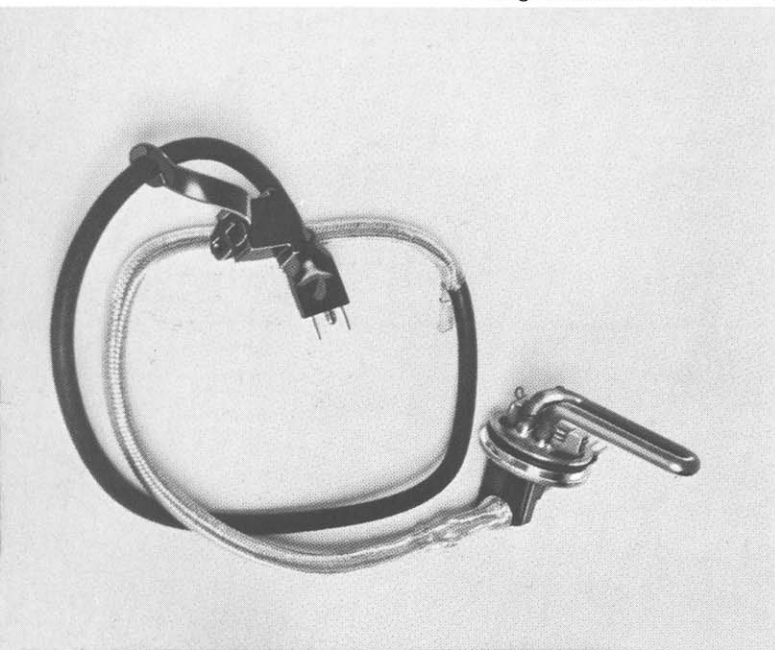
C. Engine Block Water Heater ▼
