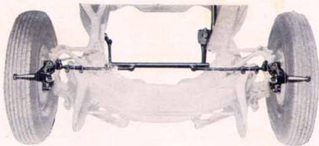
Tru-Arc Safety Steering gives positive control with minimum effort; with high steering ratio makes driving easier.
