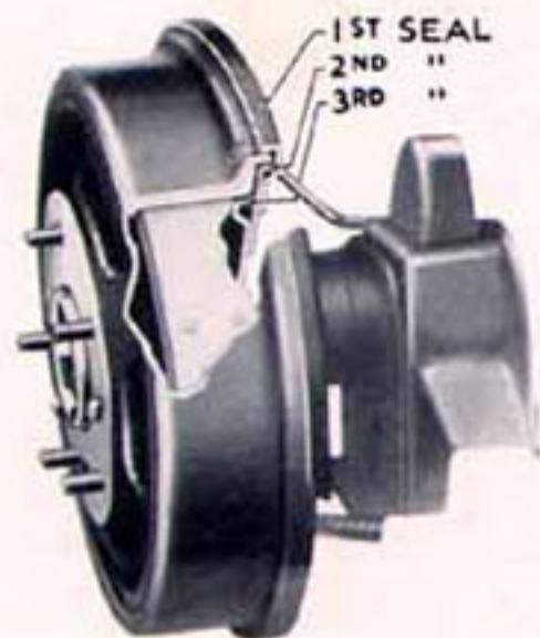
Triple-Sealed Hydraulic Brakes keep out dirt and water and are an important factor in giving you safer, surer stops in all kinds of weather.
