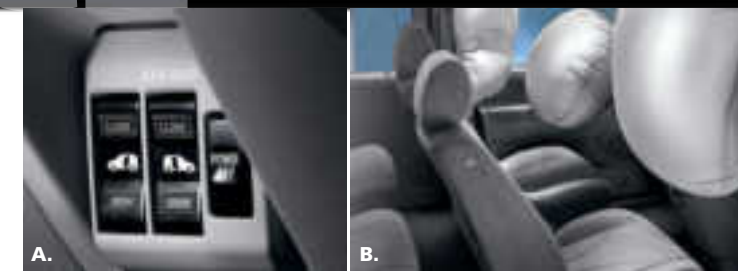
A. Power sliding doors (standard on the ES and available on the LX, not available on LX-SV) open or close at the touch of a button on the dash, door pillars or keyless entry system. A "power off" dashboard switch prevents accidental operation. B. An advanced, dual front air bag* supplemental restraint system (SRS) with crash-zone, passenger-weight and driver's seat-position sensors is standard. Dual front side-impact air bags.* (SAB) are standard on ES and optional on LX (not available on LX-SV).
