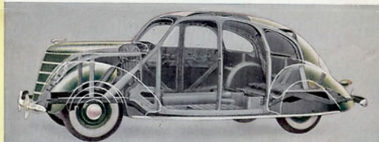
The famous LINCOLN-ZEPHYR body-and-frame, a single unit of steel girders to which steel paneling is welded. Great strength, for all its lightness, and maximum safety.
