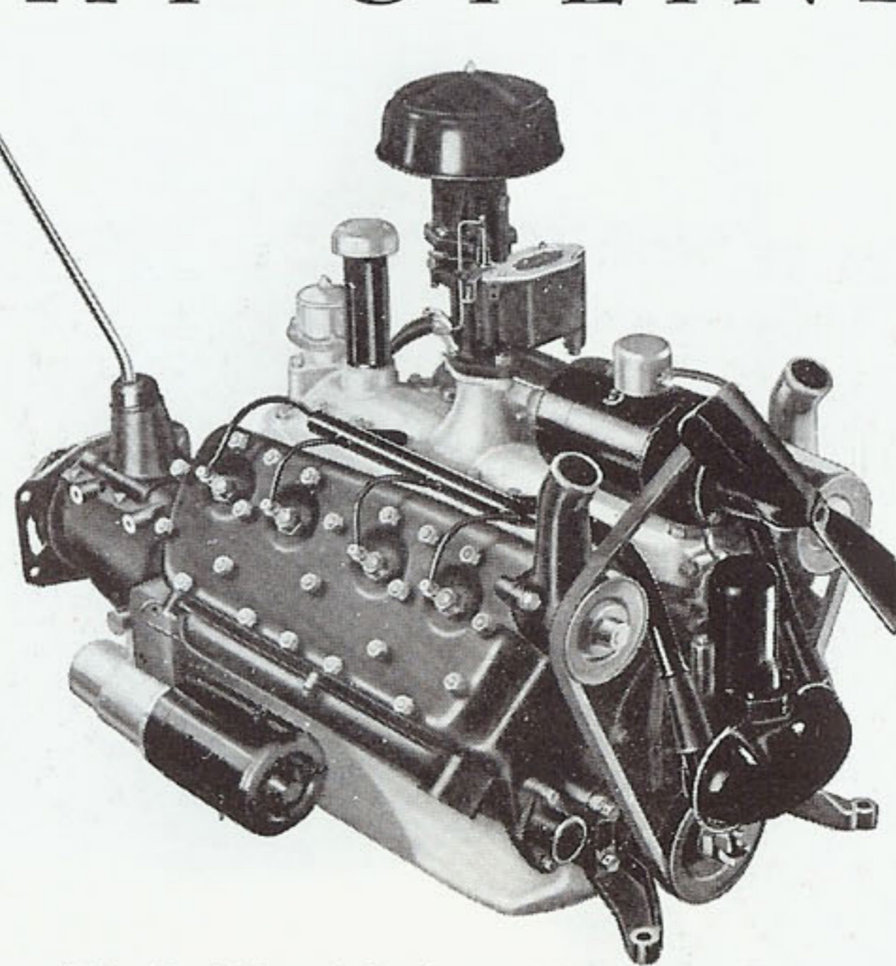
The Ford V-8 Cylinder 65 Horsepower Engine
