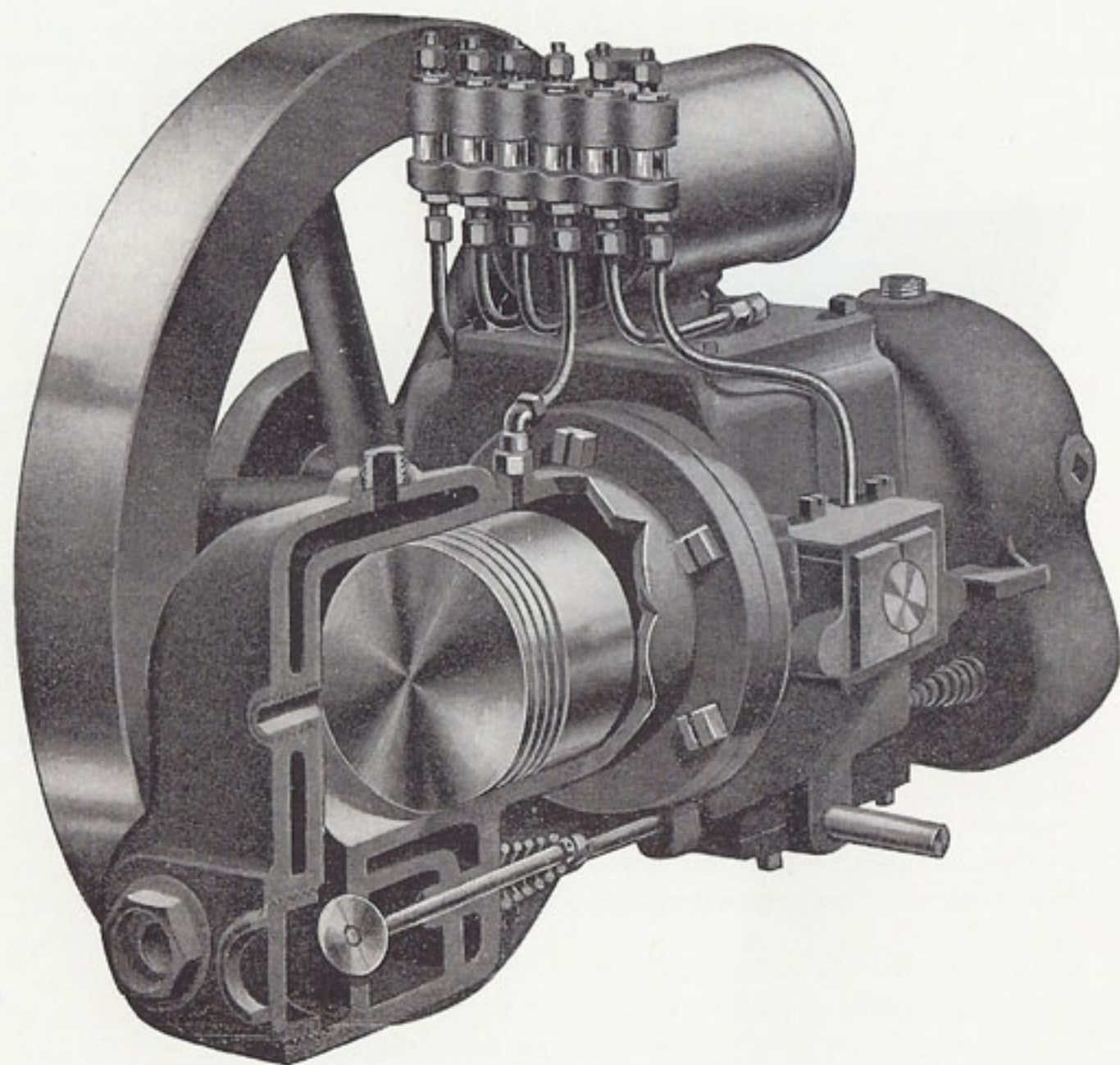
FORD OPPOSED MOTOR, MODEL C.
