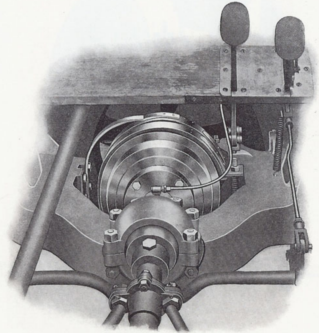
FORD MODEL B, TRANSMISSION AND GLOBE DRIVING JOINT.
