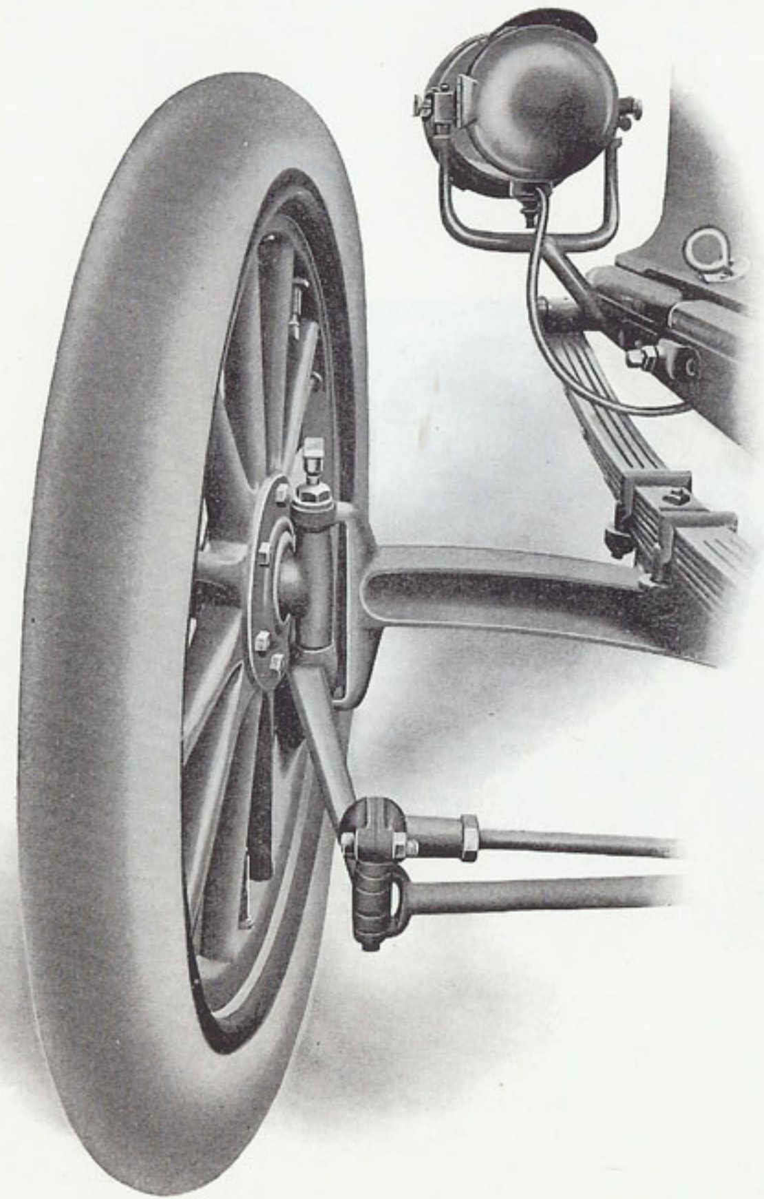
FORD MODEL B, FRONT AXLE CONSTRUCTION.
