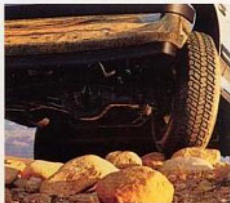
Bronco's rugged Twin-Traction Beam independent front suspension lets each front wheel step over bumps individually for a smoother ride.
