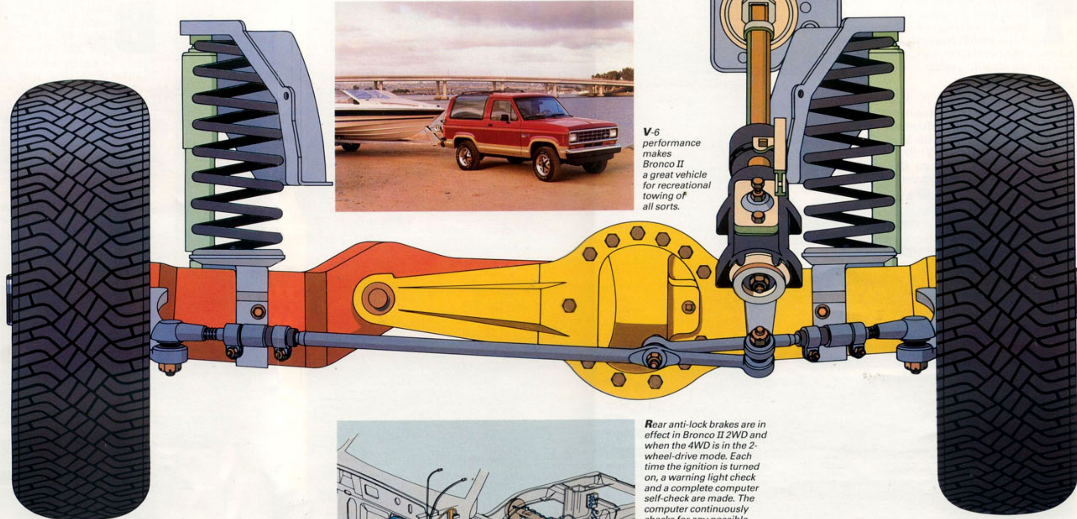
Ford-famous Twin-I-Beam independent front suspension is standard with the 2WD model and the Twin-Traction Beam system (shown above) with the 4WD. Each front wheel, with its own axle and hefty coil spring, steps over bumps independently to help cushion the ride and provide excellent handling.
