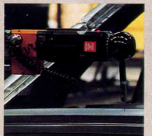
Delicate sensors on the Flexible Inspection System relay information through a computer for comparison with engineering specifications.
